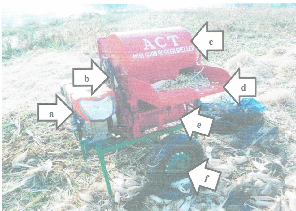
Figure 1. Parts of ACT MINI – GOLDEN BOW Corn Sheller powered by 6.0 kW GOLDEN BOW 80D1 Diesel Engine:
